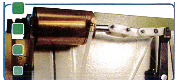
157-30 back treadle pneumatic foot lifter 157-80 Electro pneumatic foot lifter
