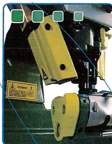
164-15 Knee press pneumatic retractable tape and chain cutter
