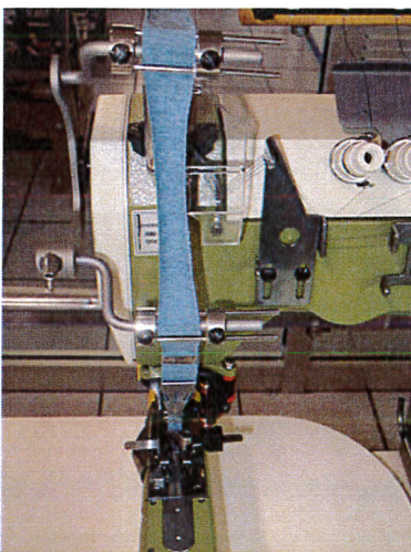
Tape rack, folder and foot
