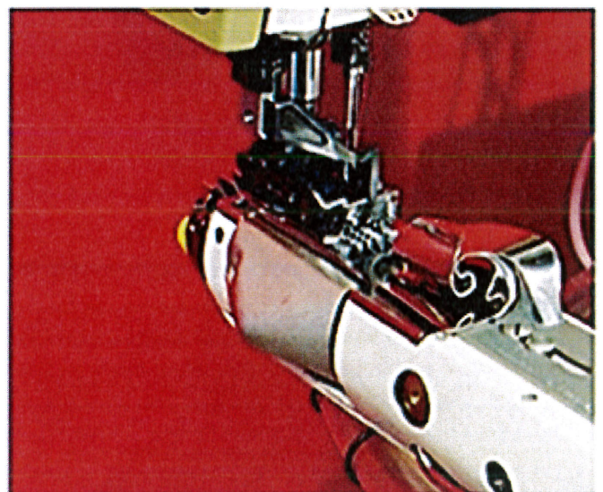
Tractor feeding foot and doublelapped folder of F84-00-2CA-11 HEAD
